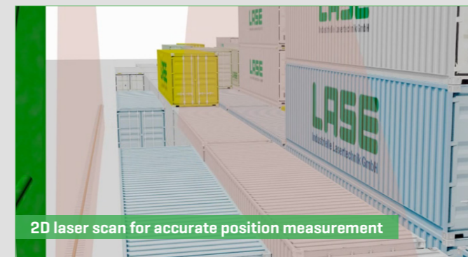
Software view - spreader approaches container load
